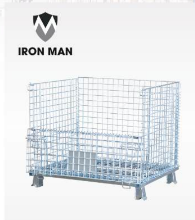
PM 5 Pallet Mesh H840 x W800 x L1000mm Capacity: 1200kg RM335
